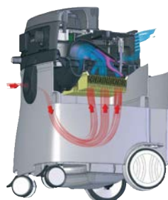
Air cycle during normal operation
